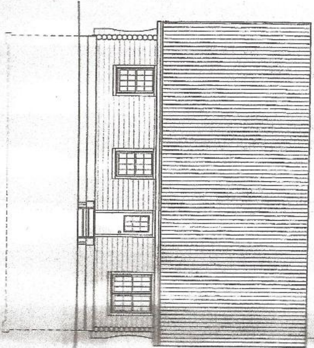
REAR ELEVATION SCALE: 1/4" = 1'-0"
