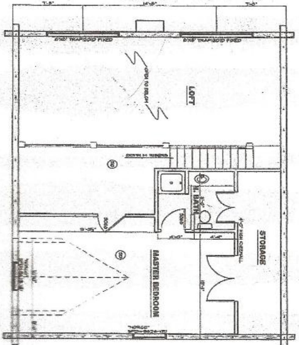
LOFT FLOOR PLAN SCALE: 1" = 1'-0"
