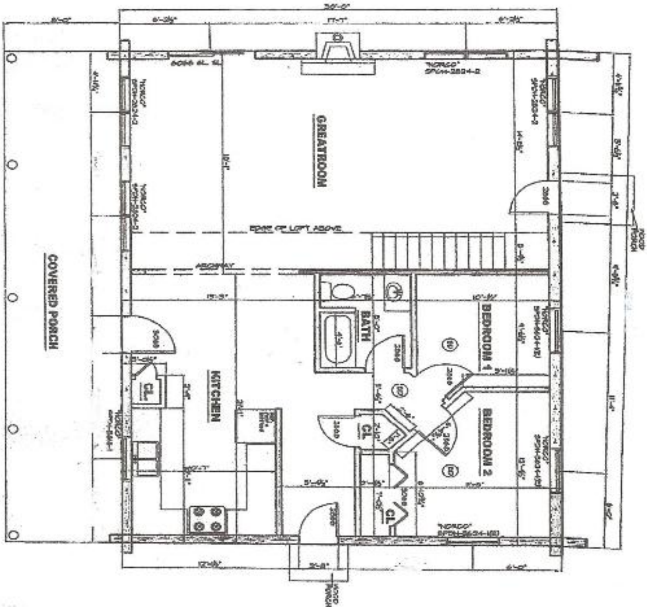
FIRST FLOOR PLAN SCALE: 1" = 1'-0"
