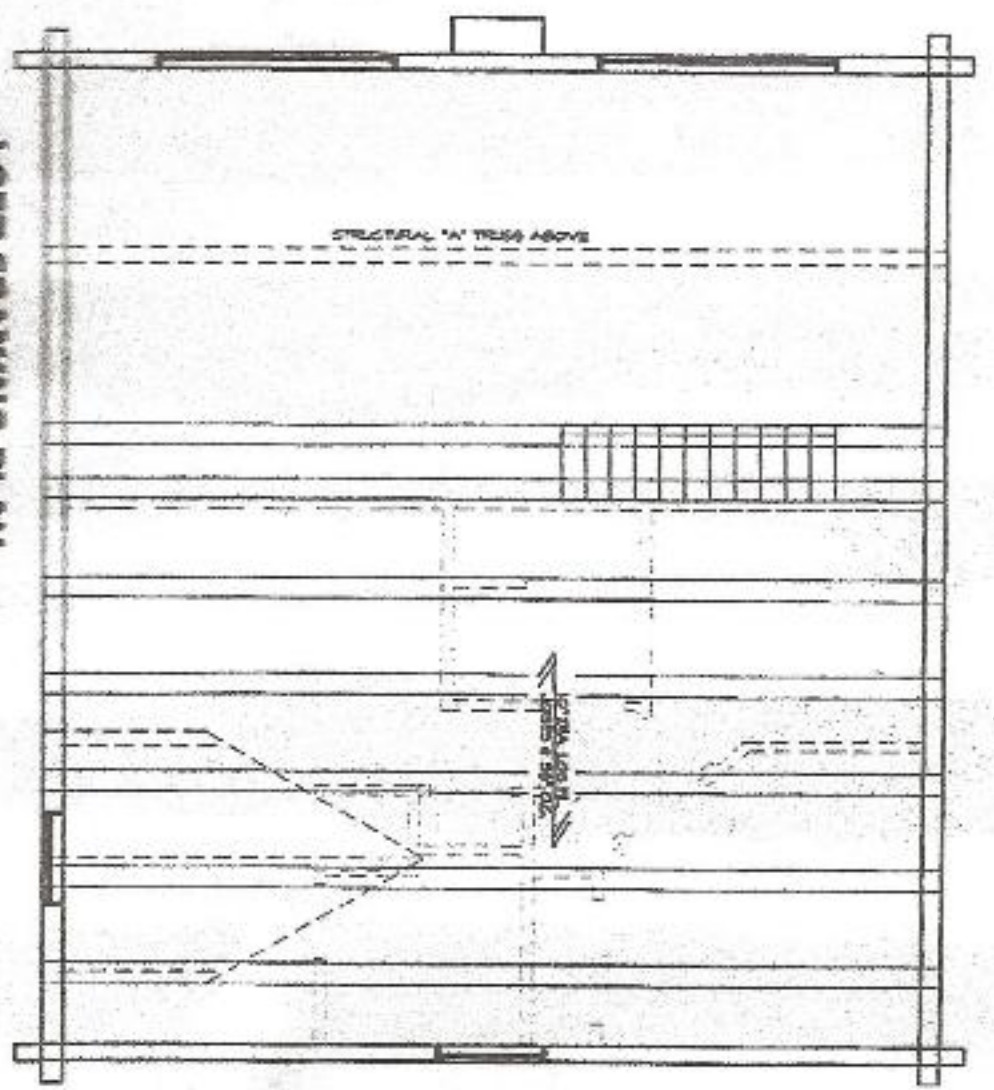
LOFT FRAMING PLAN SCALE: 1" = 1'-0"
